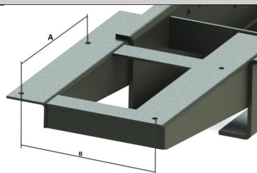
Mounting hole pattern for fitment
